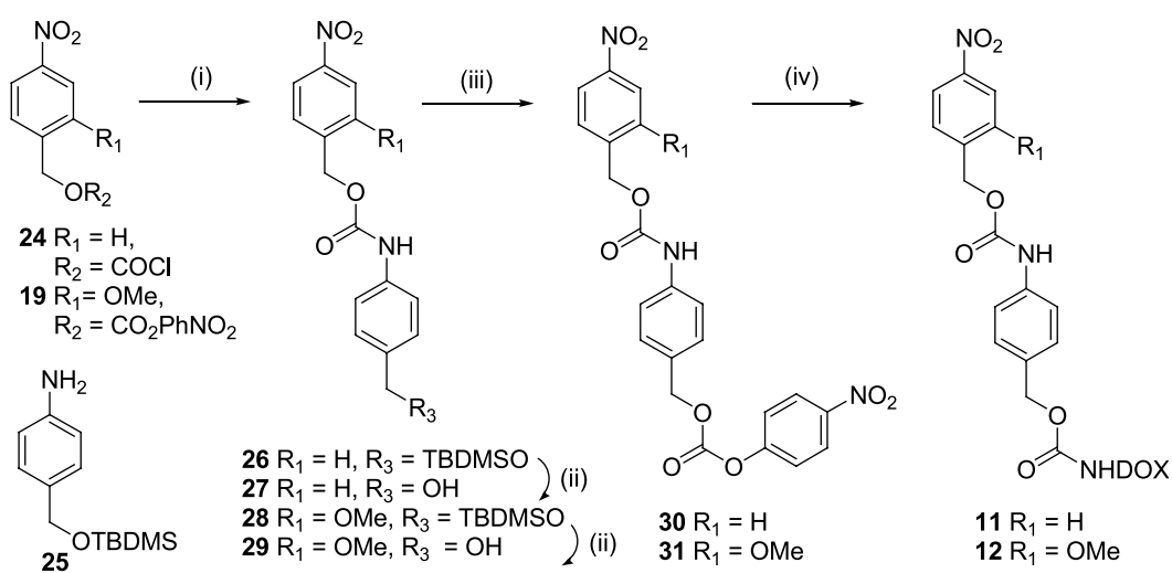
Scheme 2. Reagents: (i) (25), \text{Et}_3\text{N} , HOBT, 4 Å sieves, THF; (ii) HCl, MeOH; (iii) 4- \text{NO}_2\text{PhOCOCl} , DIEA, THF; (iv) DOX, \text{Et}_3\text{N} , DMF.
